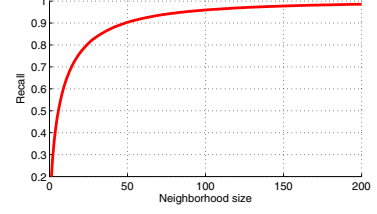
Figure 3. The coverage of the active points by the closure w.r.t. the neighborhood size. A neighborhood of size 50 has about 90% coverage.
