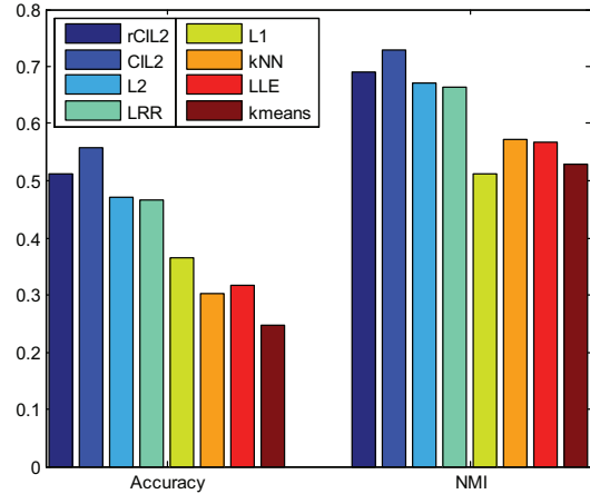
Figure 8. Clustering accuracy and NMI on the AR dataset with an unrelated image occlusion for different algorithms.
