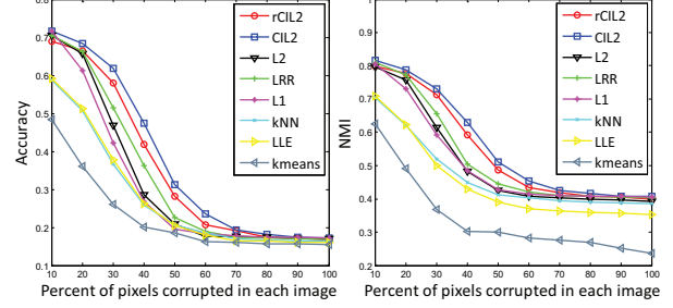
Figure 5. Clustering accuracy and NMI on the ORL dataset with pixel corruption for different algorithms.
